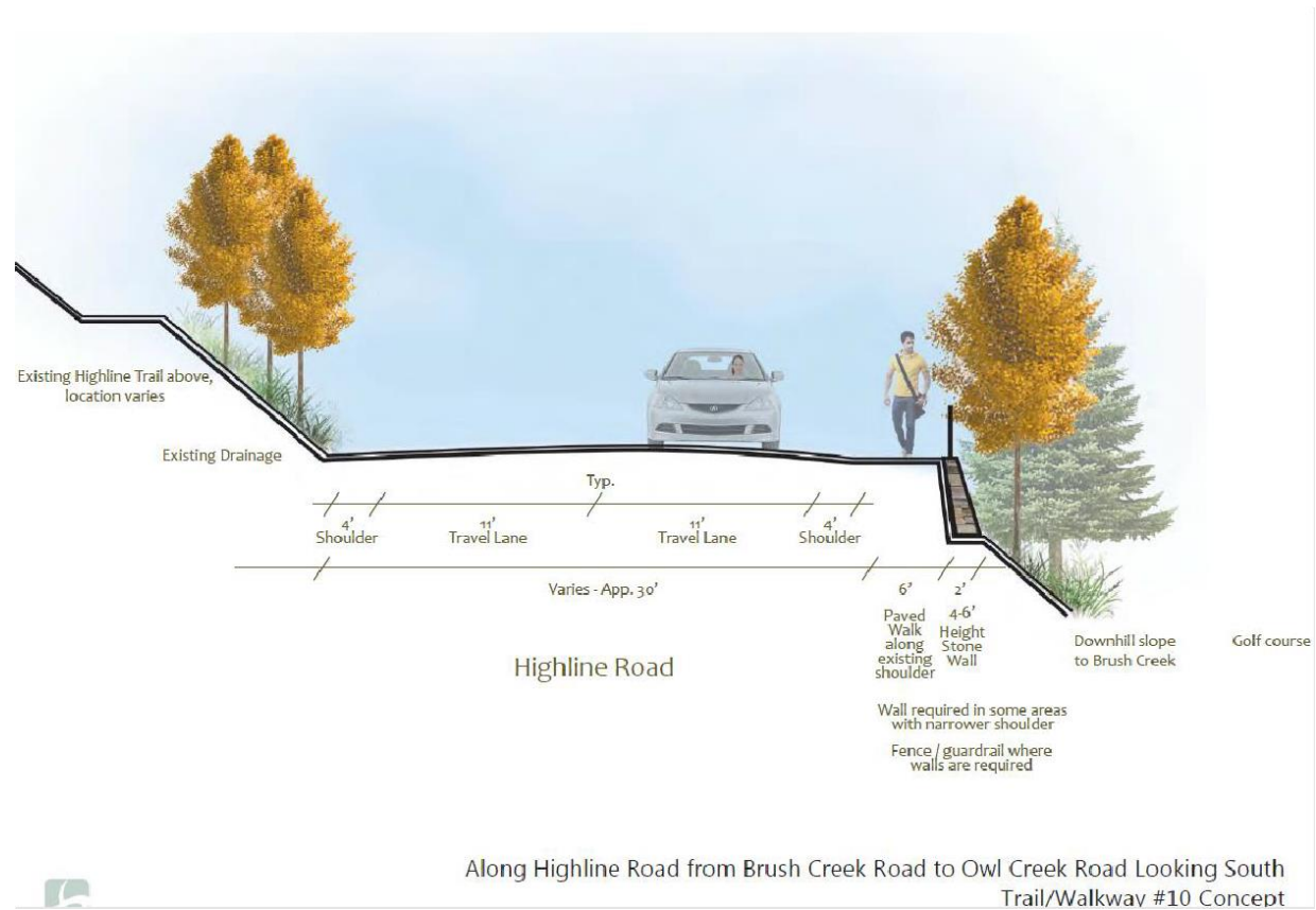
Figure 11: Walkway #10 Concept
