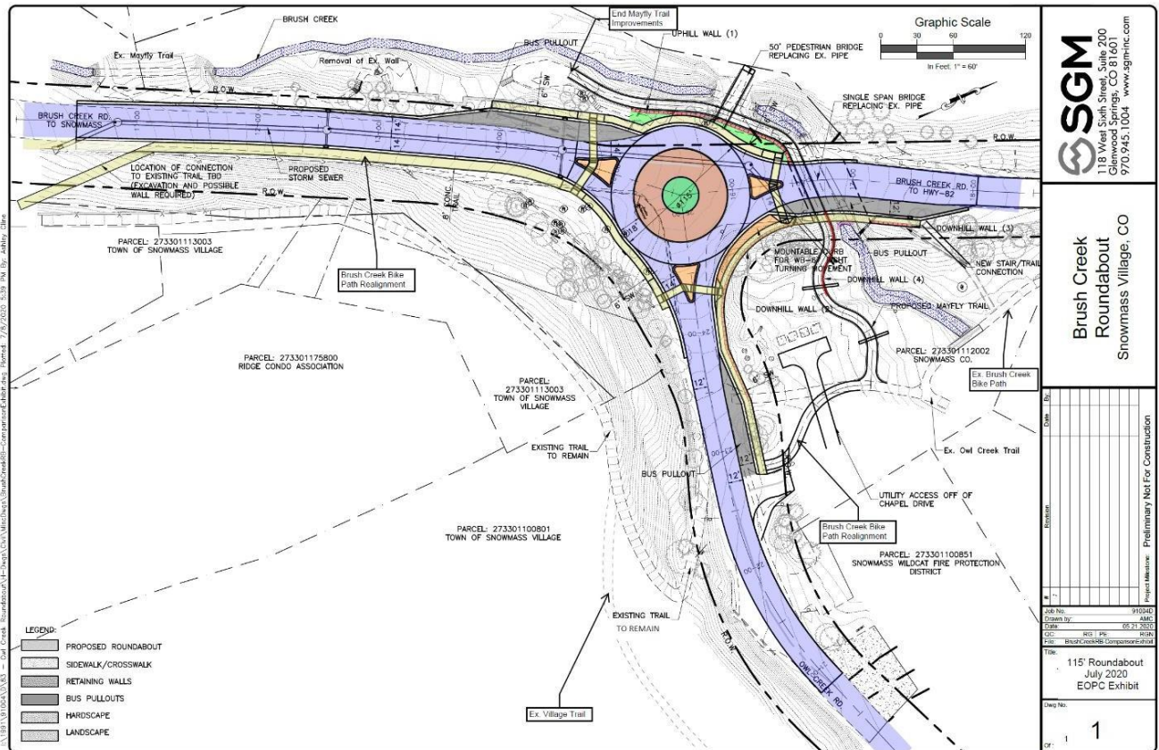
Figure 3: Proposed Intersection Improvement: Brush Creek Road/Owl Creek
