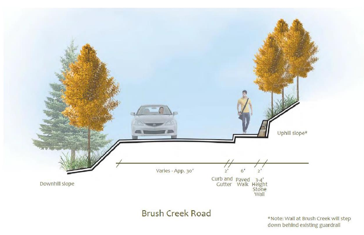
Figure 8: Walkway #3 Concept
