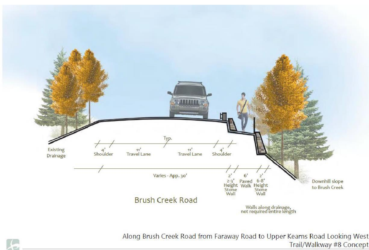
Figure 10: Walkway #8 Concept
