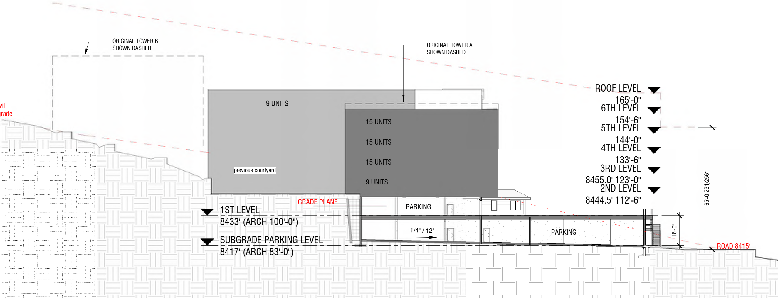
2 ONE BUILDING OPTION 6B - SECTION 1" = 30'-0"
