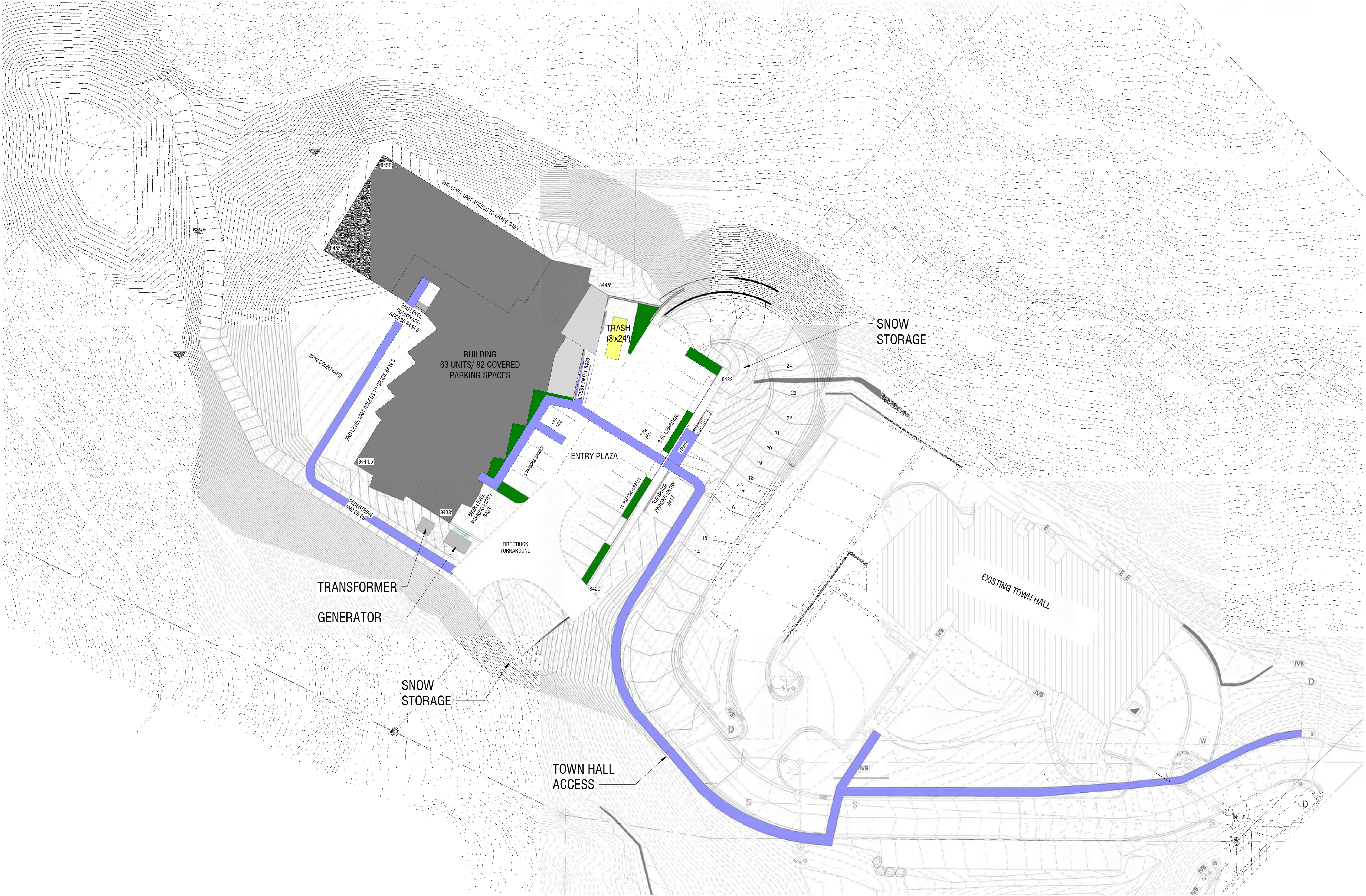
1 SITE PLAN 1" = 30'-0"
